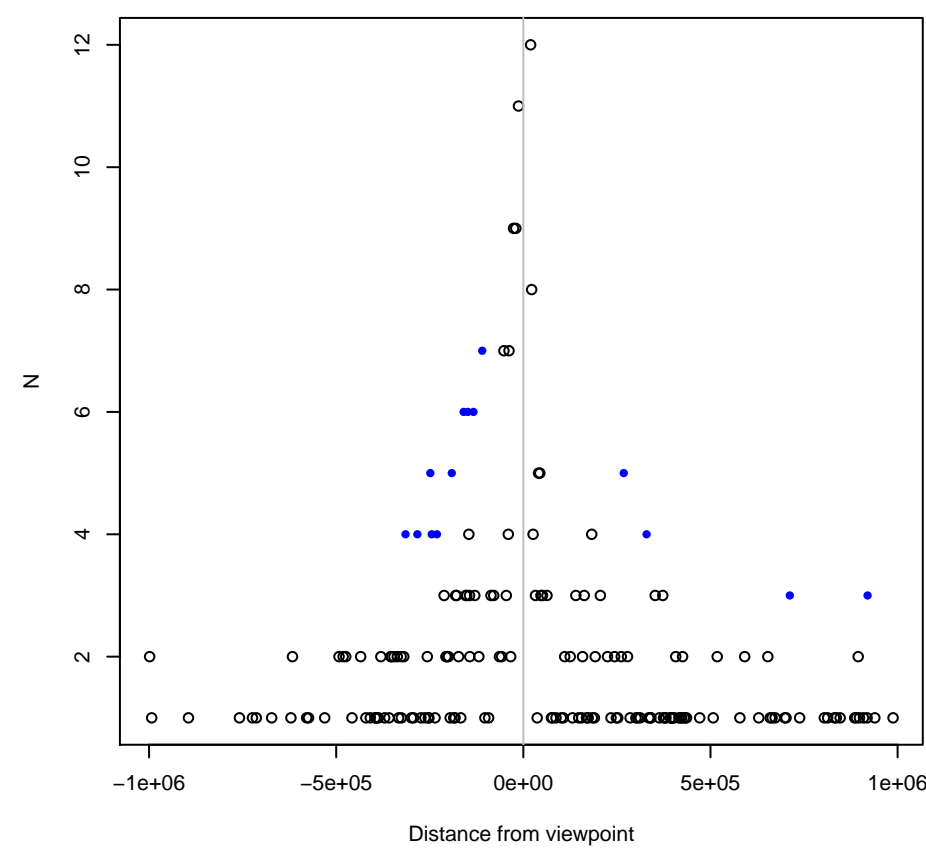
G6PD;IKBKG (829783)
