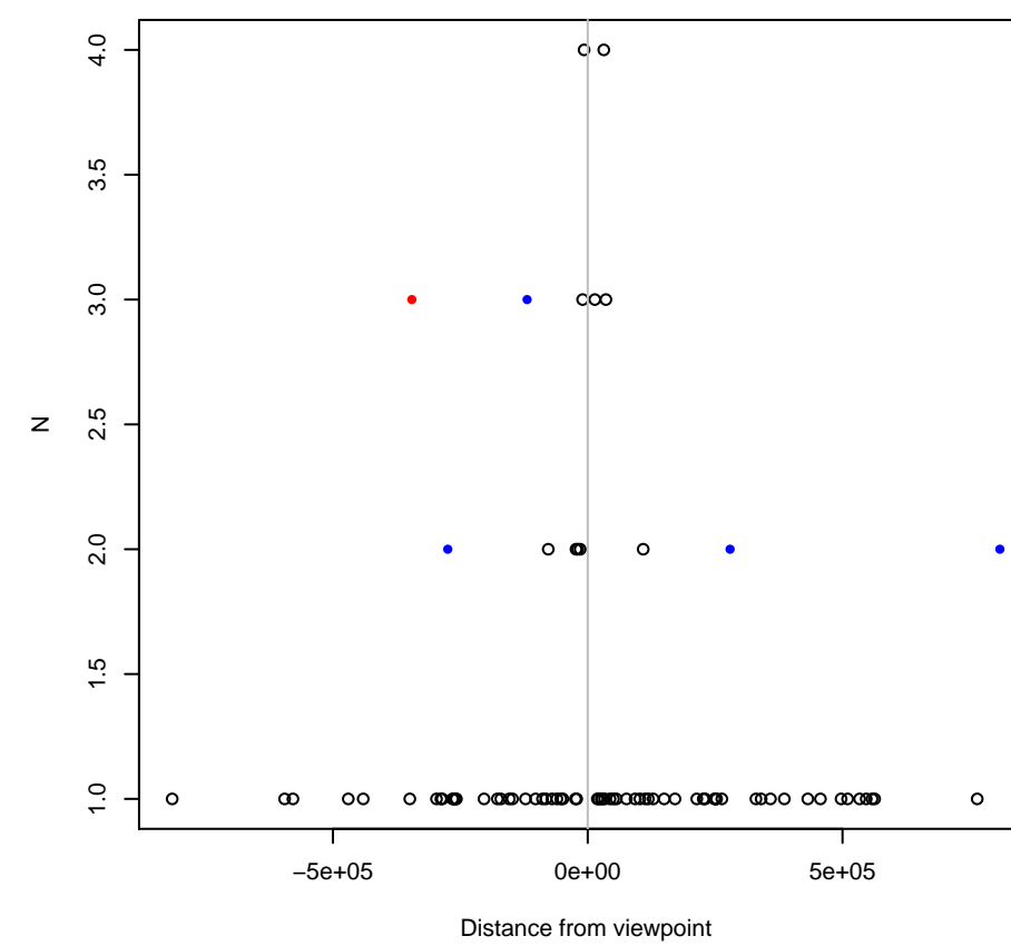
CCDC159;RAB3D;TMEM205 (322032)
