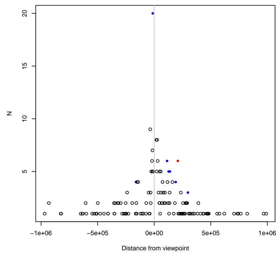
AP001053.11;RRP1;TMEM97P1 (428691)
