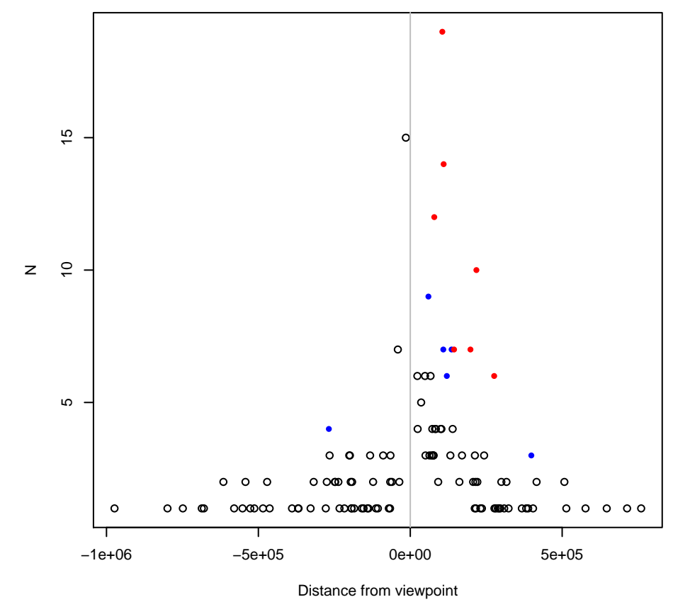
HOTAIRM1;HOXA1 (669599)
